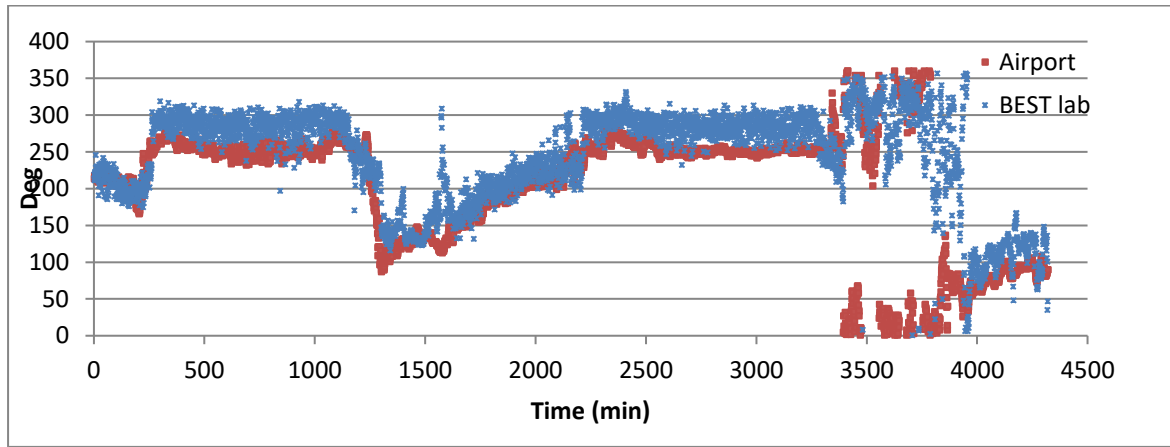
Figure 3: Wind direction
