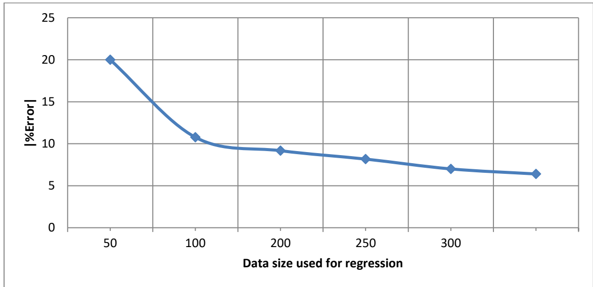
Figure 30: Impact of the data size quality on AIM-2-Regression model
